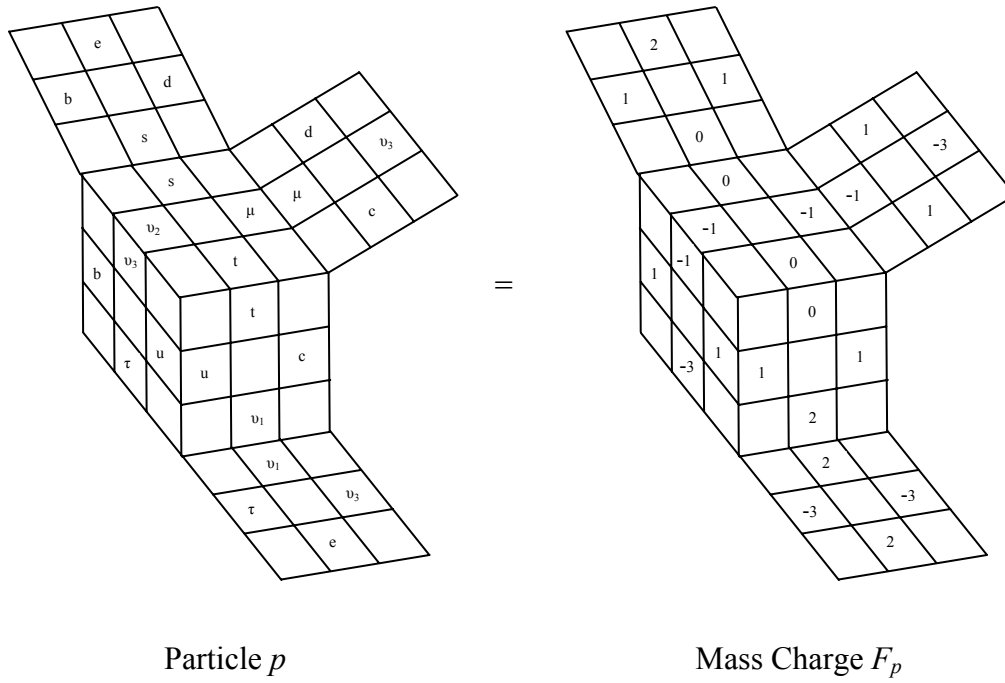
Figure 11. Assignment of mass charge F_p for quarks and leptons.
