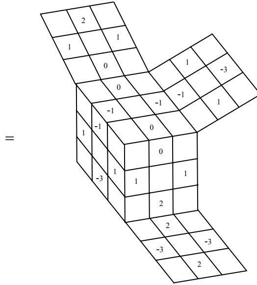
Mass Charge F_p
