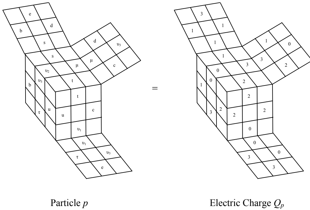
Figure 10. Assignment of electric charge Q_p for quarks and leptons.
