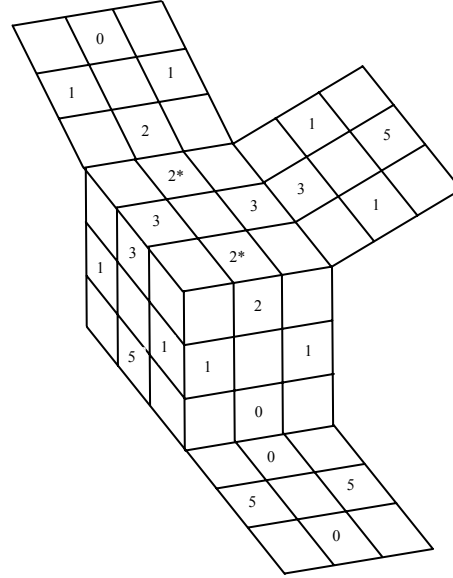
Mass Charge F'_p
