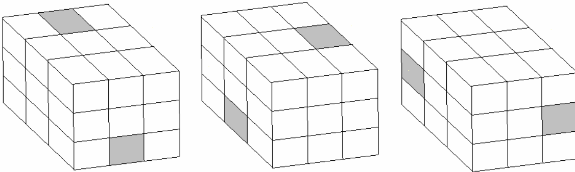
Figure 3. Examples of opposing edge-subcubes .
