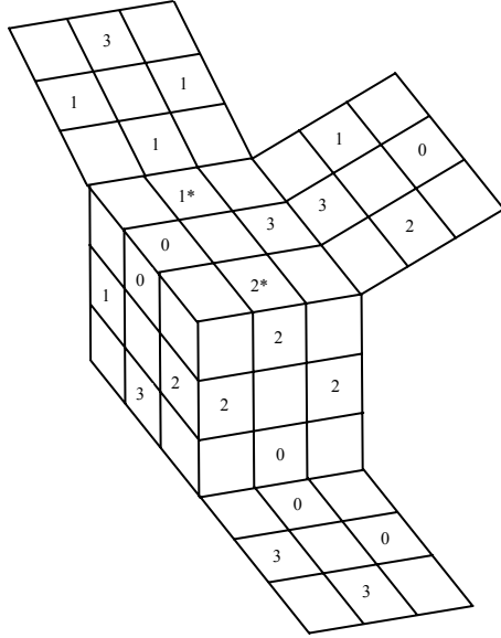
Electric Charge Q_p
