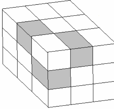
Figure 5. Example of one of the 8 corner-triads possessed by Rubik's cube.
