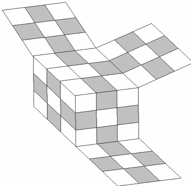
Figure 1. The 12 edge-subcubes of the 3 \times 3 \times 3 Rubik’s Cube.
