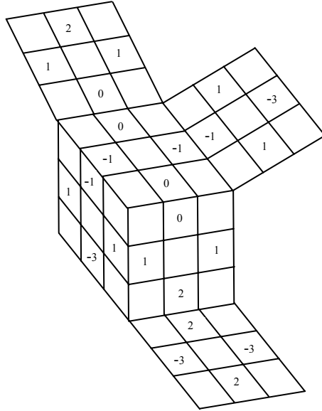
Figure 8. The mass charges F_p for the twelve quarks and leptons. Note that when the above values are divided modulo 6, and the six pairs of opposing edge-subcubes are swapped, the cube yielded is identical with that of Figure 6, which contains values for F'_p .
