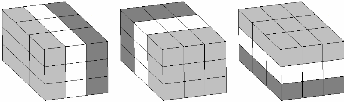
Figure 2. The 9 slices of the Rubik's Cube.
