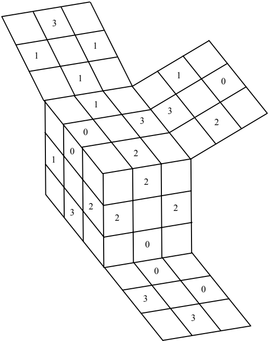
Figure 4. The arrangement of electric charge Q_p for the twelve quarks and leptons.
